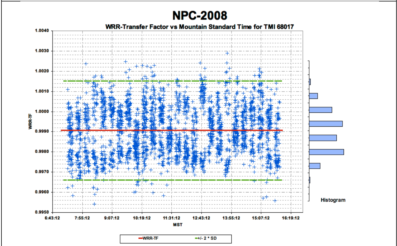
Figure 4.5.34 WRR-TF vs. Mountain Standard Time for AHF TMI 68017 at NPC-2008
